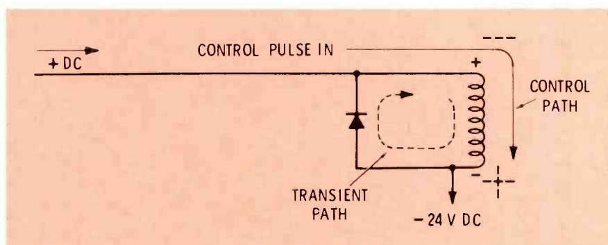
Fig. 2 The diode as a transient suppressor. Again, polarity is important. Control voltage will not pass through the diode. Transient voltage developed when control voltage is removed will be of opposite polarity, causing diode to conduct and short out the transient.
