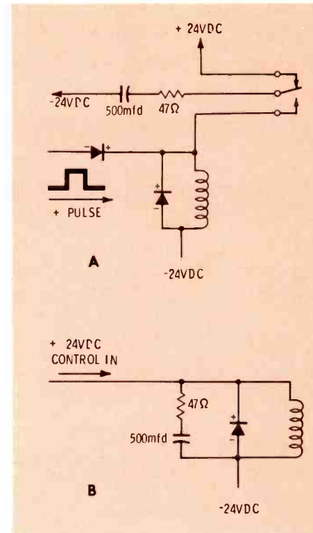
Fig. 5 A capacitor used here delays the relay drop out. Circuit A will work for a pulse input when the relay is non-latching, but is on only during pulse time. Capacitor has the effect of lengthening the pulse. Circuit B will work with a constant control voltage. With values shown, it will give about a 1 second delay.
