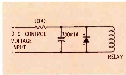
Fig. 4 A capacitor and a resistor are used here to delay the pull-in of a relay. The values shown will give about a two second delay.
